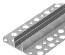
AD-LP-6504G/2M AD-LP-6504G/2M/50
