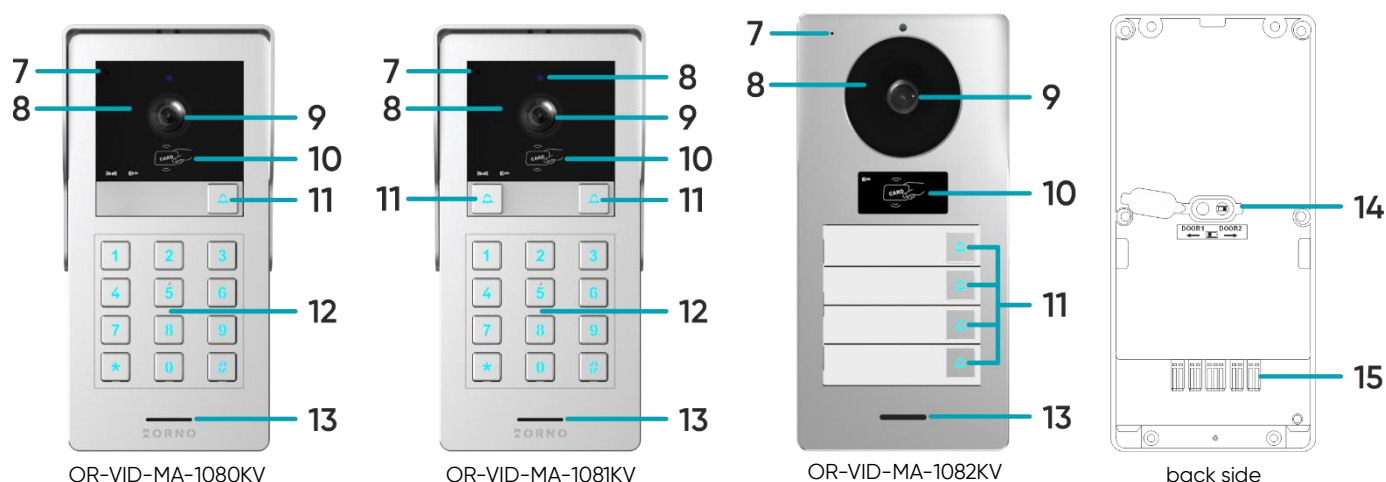
fig. 2 Construction of the outdoor unit with camera.
