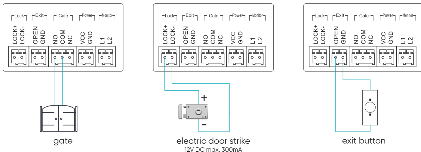
fig. 12 Gate, electric door strike, and exit button wiring scheme.
