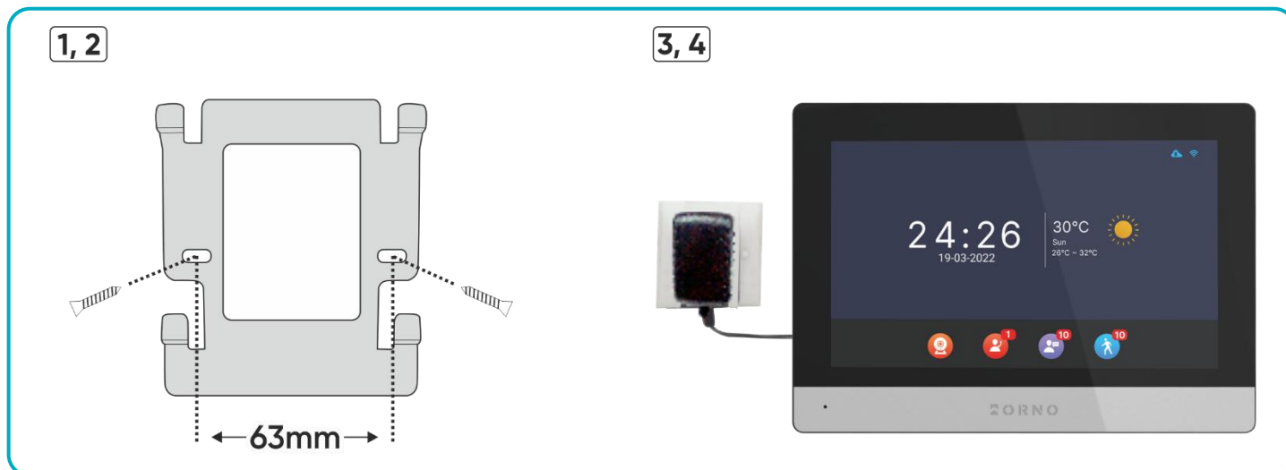
fig. 3 Monitor installation.
