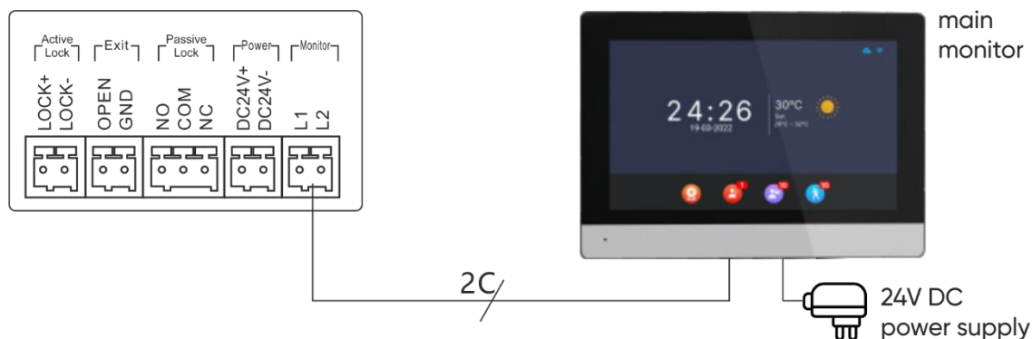
fig. 11 Monitor and outdoor unit wiring diagram.
