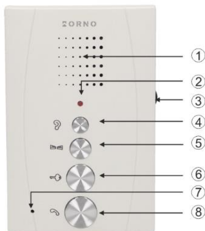
fig. 1 Indoor unit design
